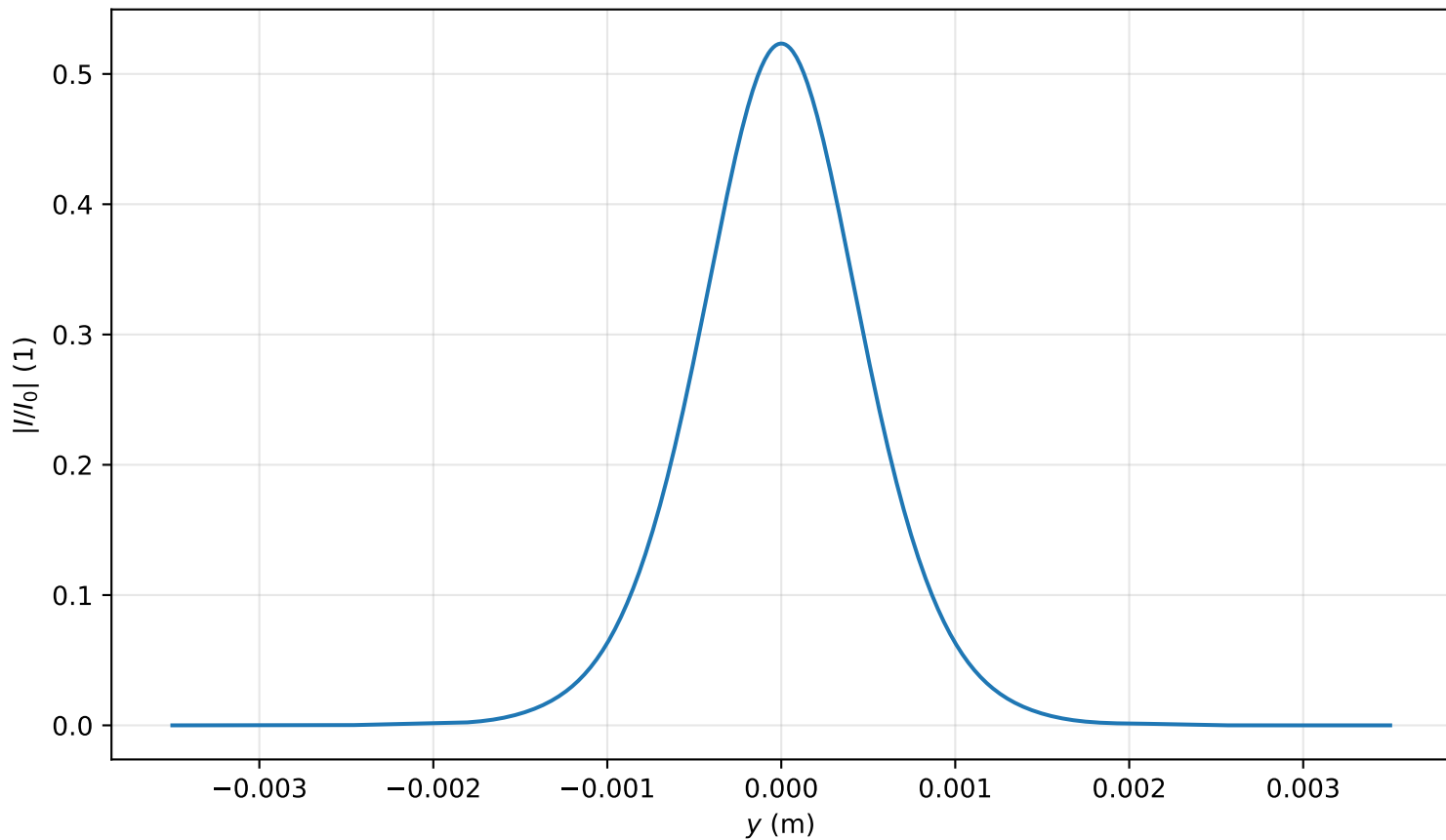
Intensity profile I(x=0, y, z=3.742)/I_0 , P_{in}=0.6P_{cr} , artificial time
